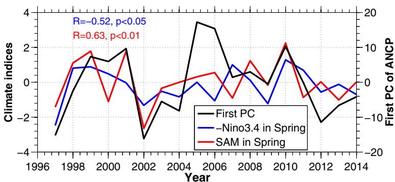
Figure 7. Correlation between the first PC of ANCP and the SAM and Niño 3.4 climate indices in austral spring. Note the reverse Niño 3.4 scale.
