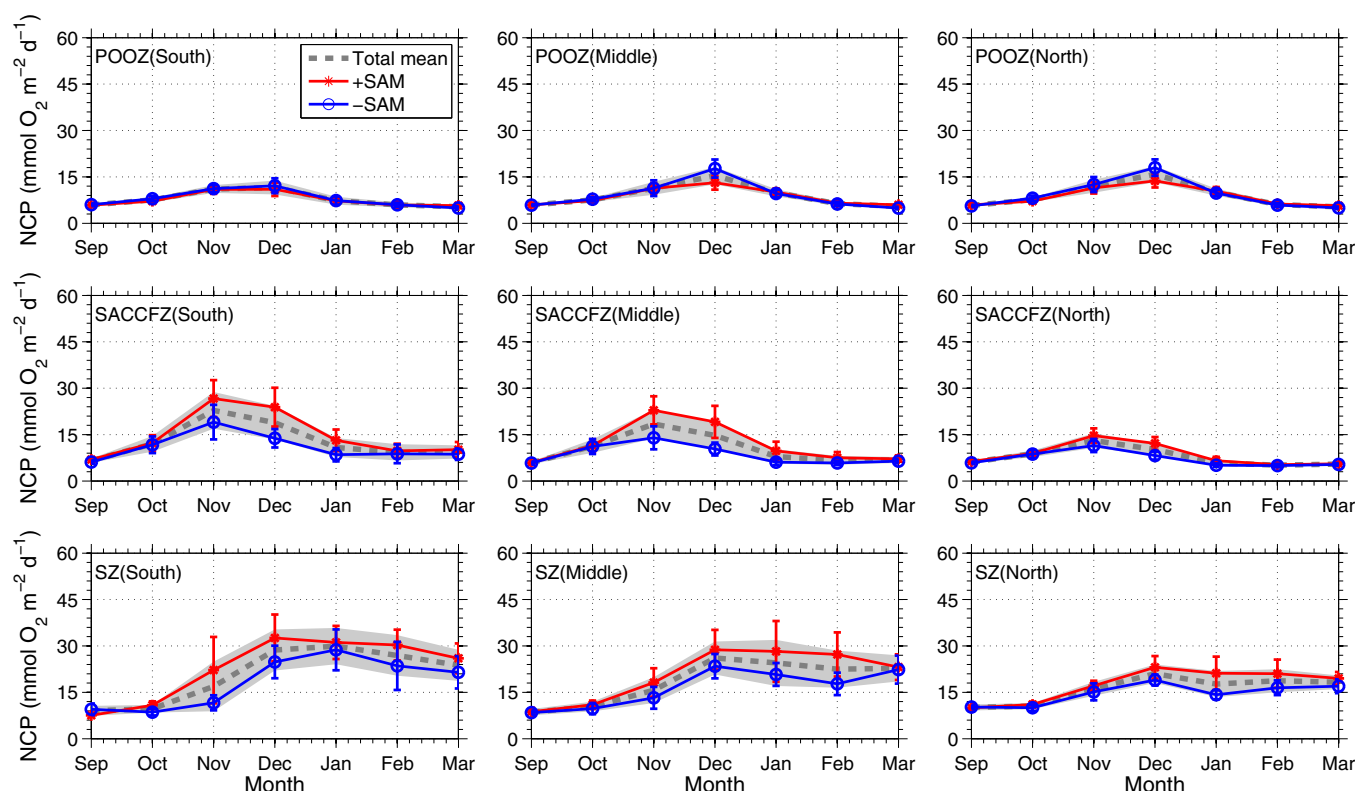
Figure 8. Multiyear arithmetic mean of MNCP in each subregion for the years with positive (1998, 1999, 2001, 2005, 2006, 2008, 2009, 2010, and 2014, red line) and negative SAM (1997, 2000, 2002, 2003, 2004, 2007, 2011, 2012, and 2013, blue line). MNCP is calculated as the geometric average of grids in each subregion. Dashed-gray line represents the climatological seasonal cycle for 1997–2014. Shaded area and the length of vertical lines represent one standard deviation.
