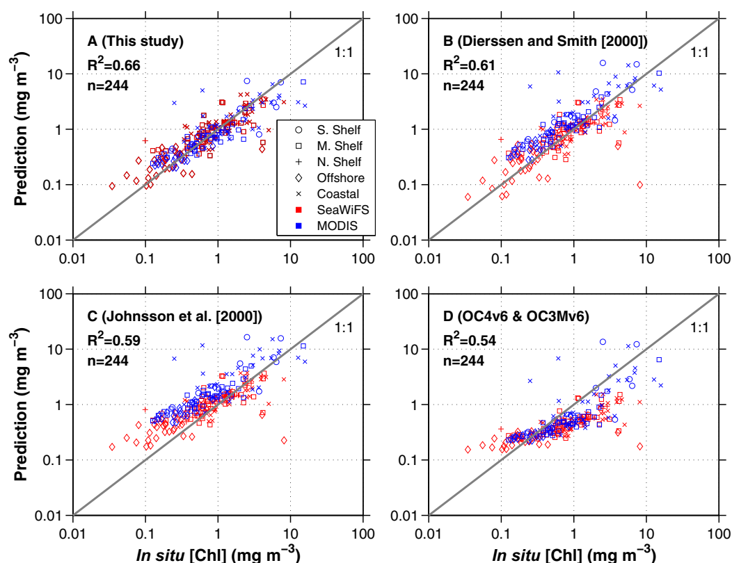
Figure 3. Comparison of in situ [Chl] to satellite (SeaWiFS and MODIS-Aqua) predictions based on (a) algorithms developed in this study, (b) Dierssen and Smith [2000]; (c) Johnsson et al. [2000]; and (d) global standard satellite-[Chl] algorithms of OC4v6 and OC3Mv6. Axes are logarithmic.
