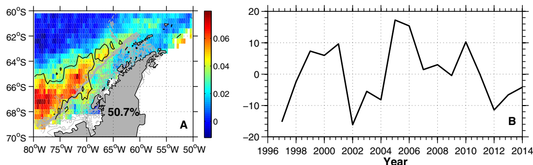
Figure 6. (a) The first EOF and (b) PC for ANCP. The high temporal variability (HTV) region is contoured in black.
