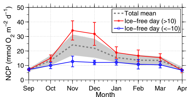
Figure 10. Multiyear arithmetic mean of MNCP in the high temporal variability (HTV) region for years with ice-free days >10 days average (1999, 2005, 2006, 2007, 2008, and 2010, red line) and <-10 days average (2001, 2002, 2003, 2004, and 2012, blue line). Dashed-gray line represents climatology for 1997–2014. Shaded area and the length of vertical lines represent one standard deviation.
