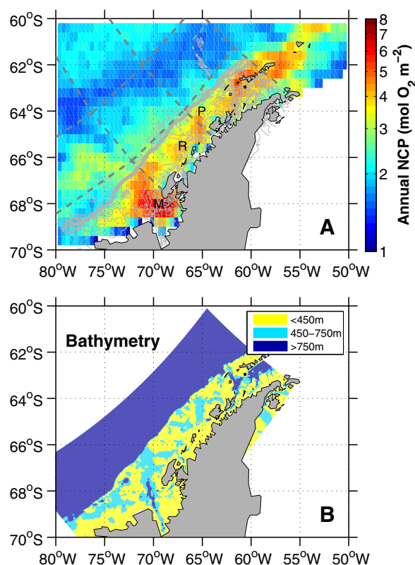
Figure 5. (a) Climatology of ANCP calculated from 1997 to 2014 time series and (b) color-coded bathymetry for the WAP region. Thin gray lines represent 250 m-increment isobaths, which collapse into a thick gray line at the shelf break. Gray dashed line separates the WAP region into nine subregions as defined in Figure 1. Letters P, R, and M identify Palmer deep, Renaud canyon, and Marguerite Trough, respectively. White area is covered by sea ice/cloud. NCP is on a logarithmic scale.
