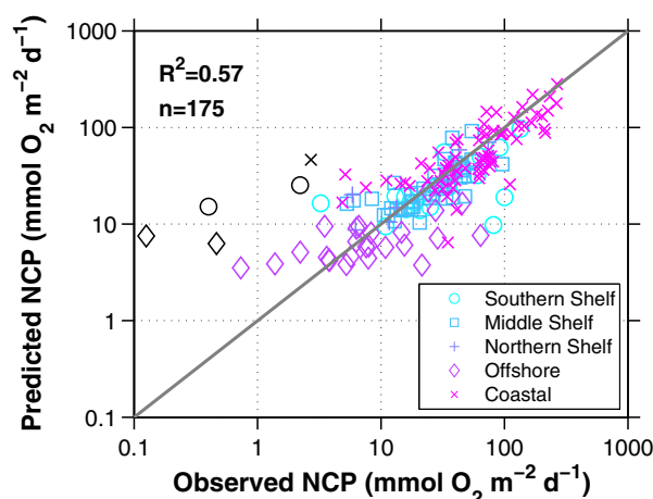
Figure 2. O_2/Ar -NCP measurements and predictions by the Bayesian hierarchical algorithm. “Coastal” represents region \leq 50 km from the coast. Axes are logarithmic.
