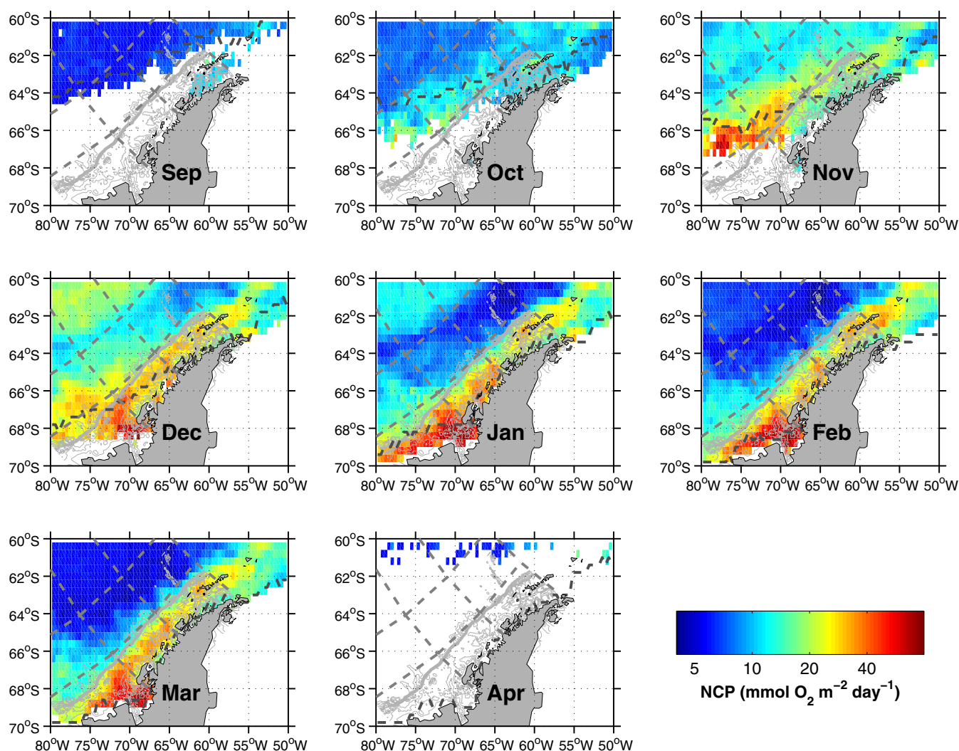
Figure 4. Climatology of MNCP derived from 1997 to 2014 time series. Thin gray lines represent 250 m-increment isobaths, which collapse into a thick gray line at the shelf break. Thick black-dashed line is the climatological ice edge for that month from 1990 to 2012. Gray dashed line separates the WAP region into nine subregions as defined in Figure 1. White area is covered by sea ice/cloud. NCP is on a logarithmic scale.
