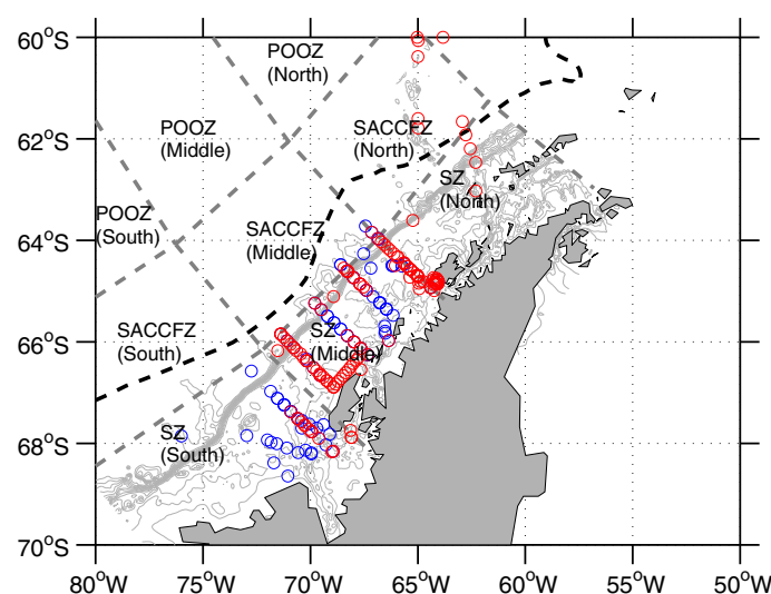
Figure 1. Study area (extended Pal-LTER region). Red and blue symbols represent the locations of in situ [Chl] samples matched to SeaWiFS and MODIS-Aqua observations, respectively. Heavy dashed line is the approximate location of the Southern Antarctic Circumpolar Front (SACCF) [Orsi et al., 1995]. Gray dashed line separates the WAP region into nine subregions. Thin gray lines represent 250 m-increment isobaths, which collapse into a thick gray line at the shelf break (750 m deep).
