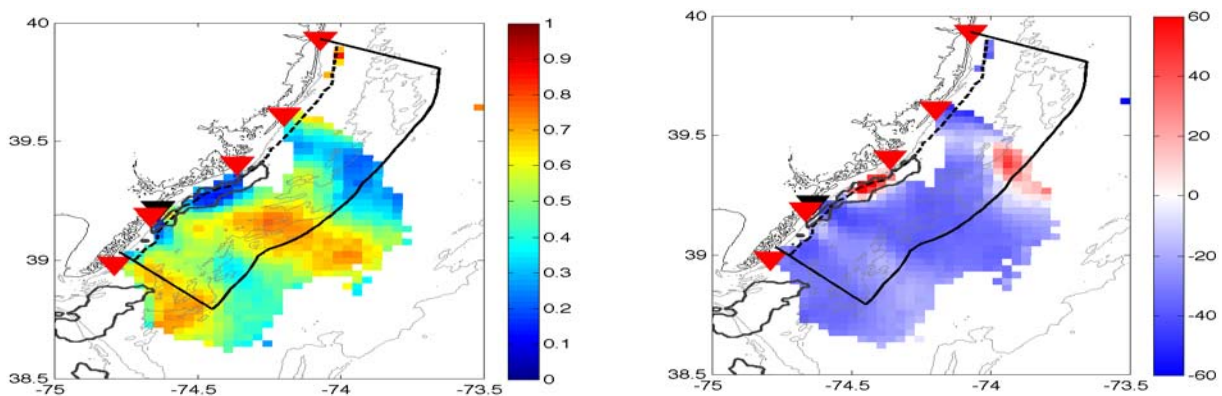
Figure 22: Magnitude of complex correlation (left) and angle offset (right) between the CODAR-predicted surface wind and RUWRF modeled 10m wind, for the upwelling case. Black triangle: location of the Ocean City Weatherflow site; Red triangles: 13 MHz CODAR sites; Black solid line: study area coinciding with NJ DEP's OSWEBS area; Dashed line: boundary between federal and state waters; Gray solid contour: 22^\circ\text{C} isotherm of SST, showing coastal upwelling in the study area.
