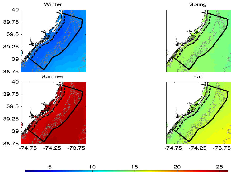
Figure 15: Seasonal SSTs (°C) in the study area from 01 January 2012 through 17 December 2012. Data are displayed using a single scale from 2°C to 26°C to provide an overview of the SSTs in relation to season.
