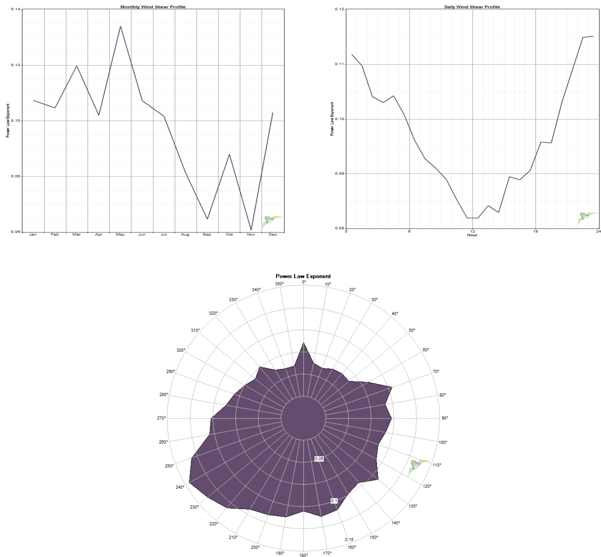
Figure 49: Virtual meteorological tower C3: (a) upper left, monthly wind shear; (b) upper right, diurnal wind shear; (c) lower left, wind shear by direction (winds coming from the designated direction).
