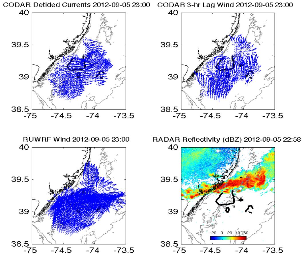
Figure 24: De-tided surface currents on 5 Sep 2012 23:00 GMT (top left), wind predicted for 23:00 GMT based on the currents 3-hrs earlier (top right), RU-WRF model 10m wind at 23:00 (bottom left), and weather radar reflectivity depicting a line of strong thunderstorms at 22:58 GMT (bottom right). Black contour: greater than 0.65 correlation between CODAR-derived surface winds and RU-WRF model 10m winds during the entire non-upwelling case.
