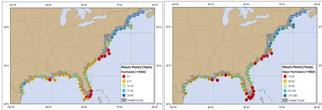
Figure 50: (a) Hurricane and (b) Major Hurricane Return Period (years) from the National Hurricane Center.
