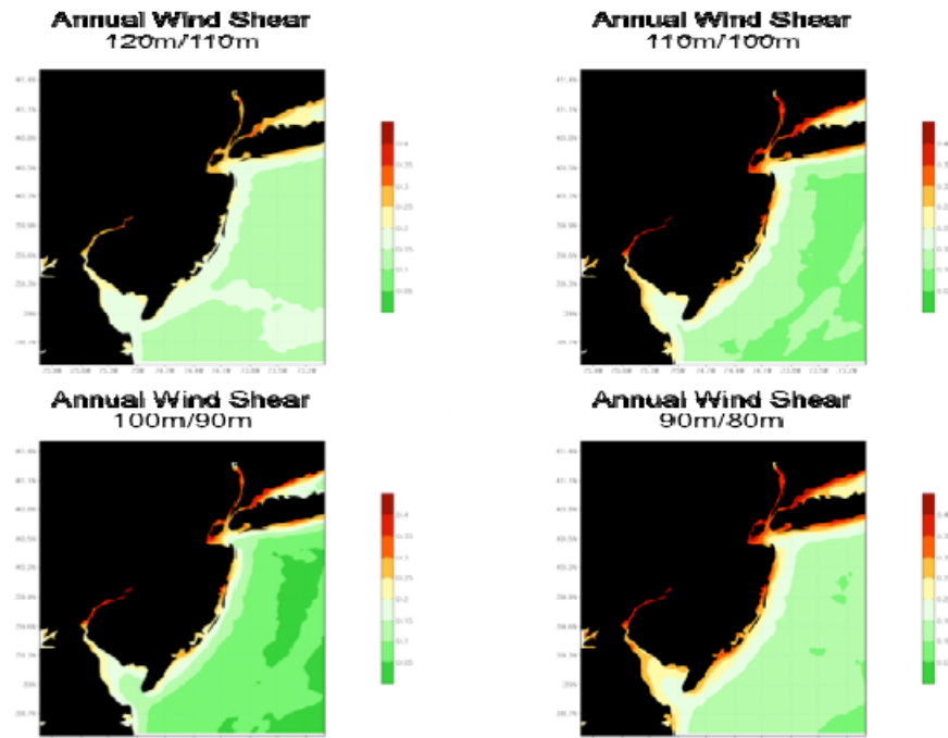
Figure 48: Annual average wind shear between (a) Upper left, 120m and 110m (b) upper right, 110m and 100m (c) lower left, 100m and 90m (d) lower right, 90m and 80m.
