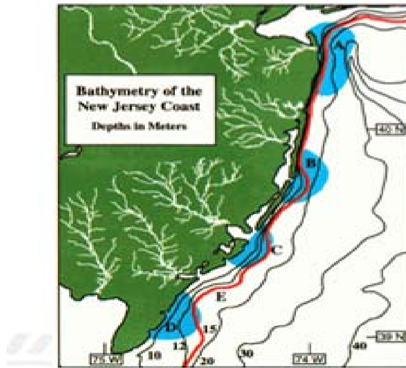
Figure 5: NJ Coastal Upwelling Centers
