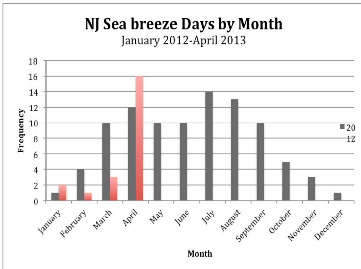
Figure 62: New Jersey sea breeze days by month, as determined using KDIX weather radar. Several more sea breezes occurred in February/March 2012 vs. February/March 2013 (14 vs. four), possibly due to a warmer than average late winter and early spring in 2012 and an average to colder than average late winter and early spring in 2013.
