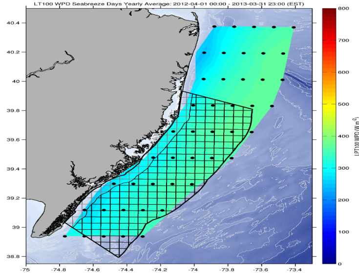
Figure 63: Average wind power density at the 100m height for sea breeze events that occurred from 1 Apr 2012 to 31 Mar 2013. Black dots: virtual meteorological towers; Black outline: 2010 NJ DEP OSWEBS area extending 20 nm offshore; Thin Black line: federal-state waters boundary line at 3 nm offshore; Black and Gray grid: federal and state offshore lease blocks.
