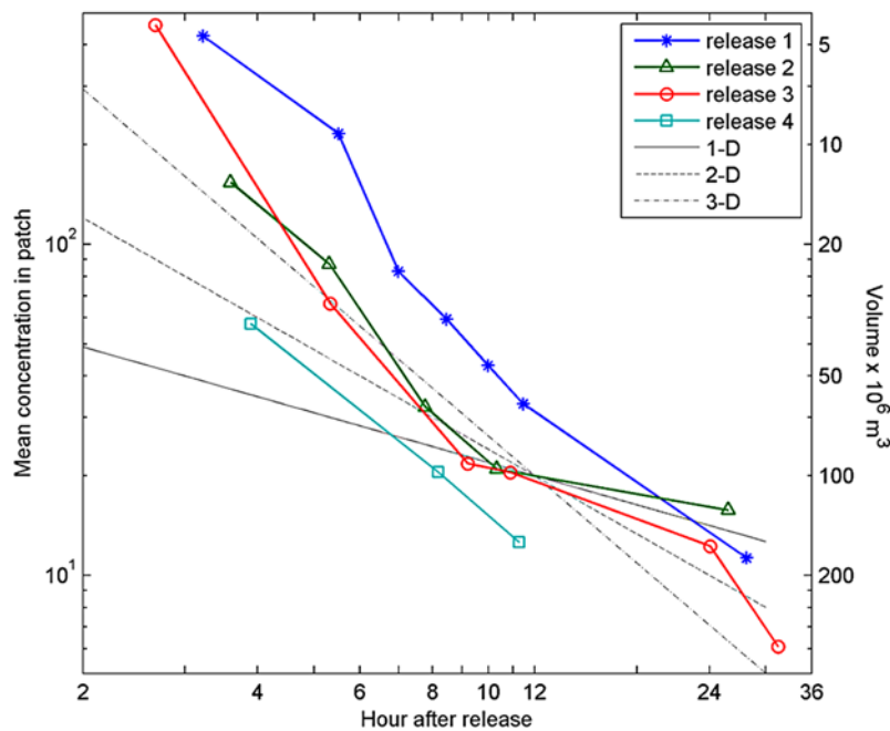
Figure 6. Patch-averaged dye concentration (units 10^{-8} kg/m 3 ; left axis) for all 4 releases as a function of time since the release. The equivalent volume of the patch is shown on the right. Also shown are lines of constant dilution rate for 1-dimensional, 2-dimensional and 3-dimensional spreading.
