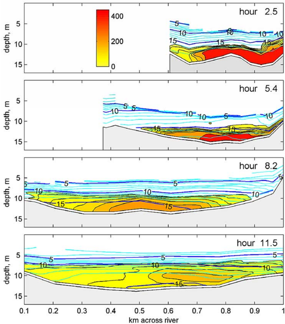
Figure 4. Cross-sections across the estuary at various times following the 1st release. Dye and salinity contours are shown as in Figure 3. Each cross-section is roughly in the center of the patch.
