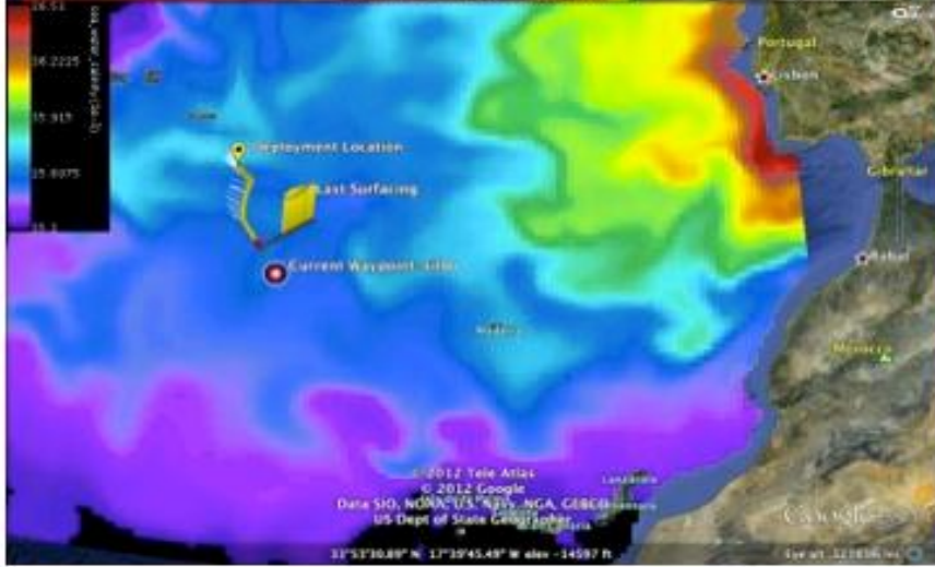
Salinity 900m
