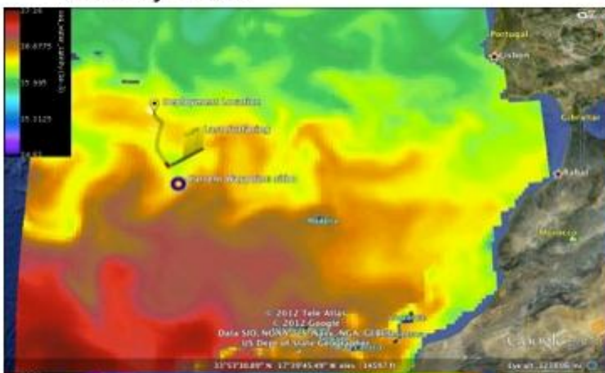
Salinity 100m
