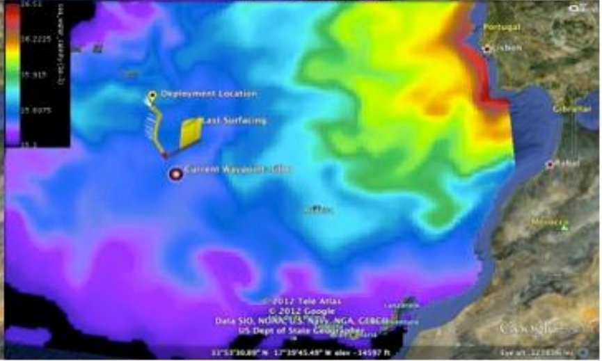
Salinity 1000m
