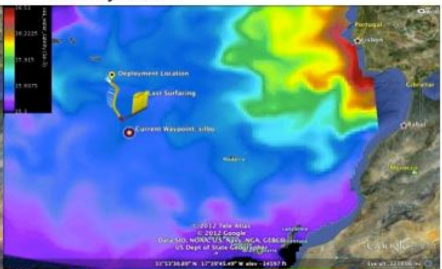
Salinity 600m
